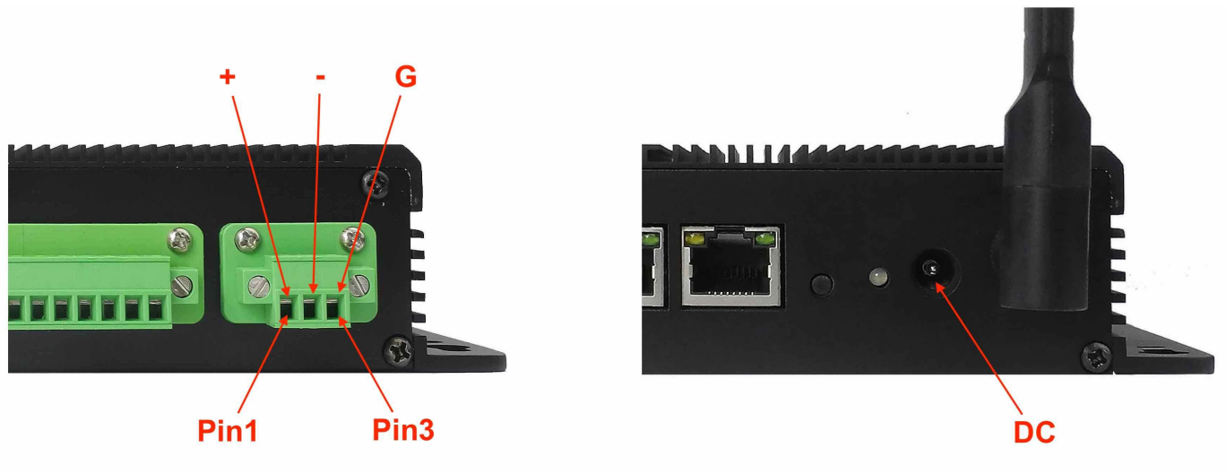
Power Input
