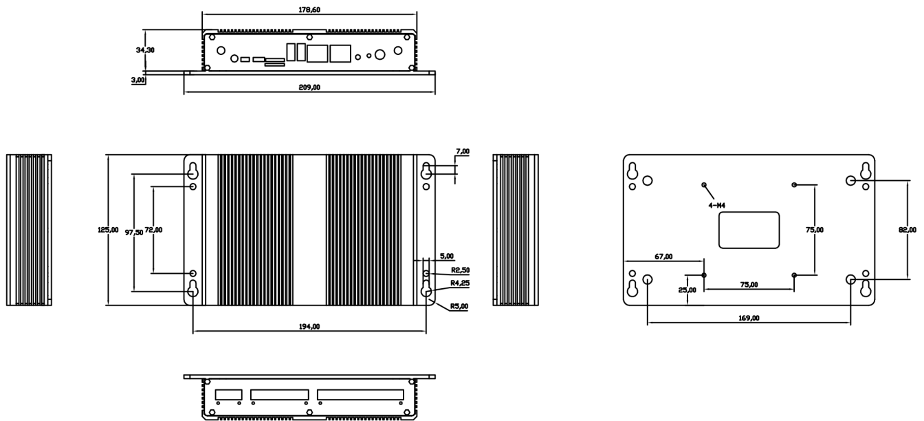
Figure 668: CS-A55-BOX Technical Drawing
