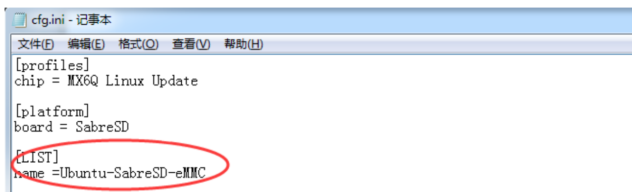
Figure 263: Cfg.ini file
