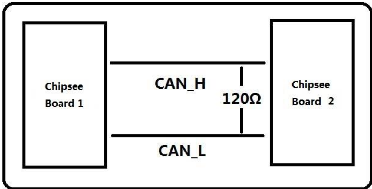
Figure 280: CAN Connect
