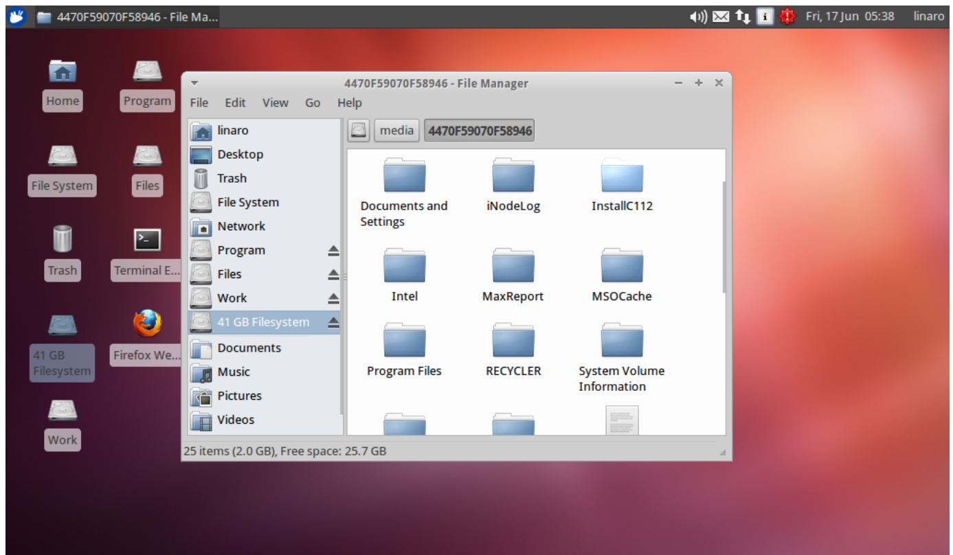
Figure 276: SATA test
