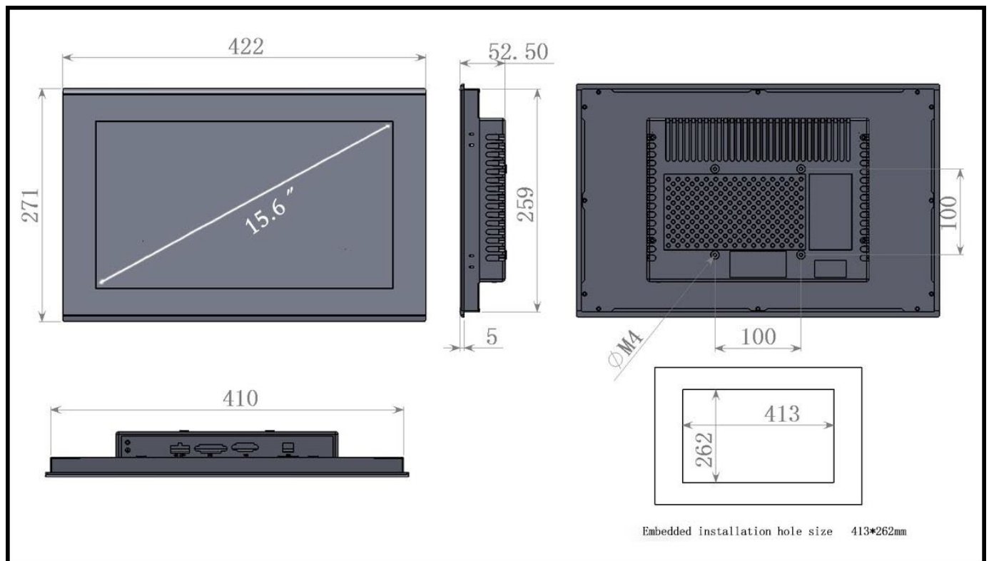
Figure 897: PPC-J1900-156-C Technical Drawing
