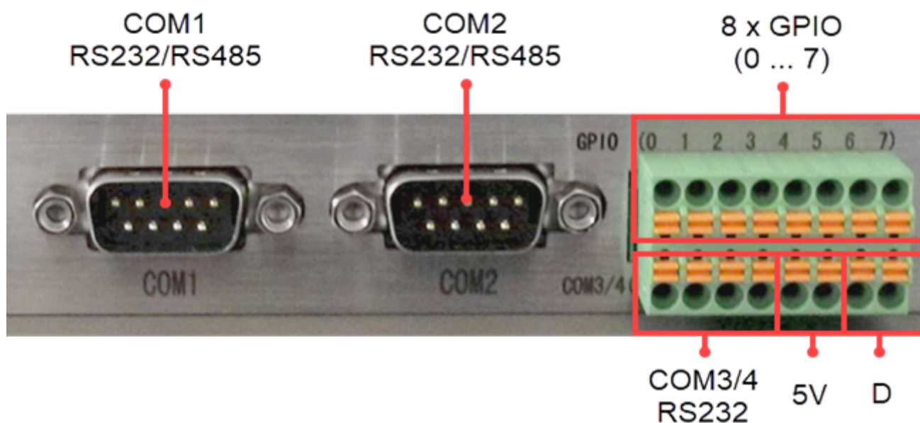
Figure 893: Figure 2: Connectivity Section - 2 x D-sub Connectors & 16-pin Double-Row Pluggable Terminal Block
