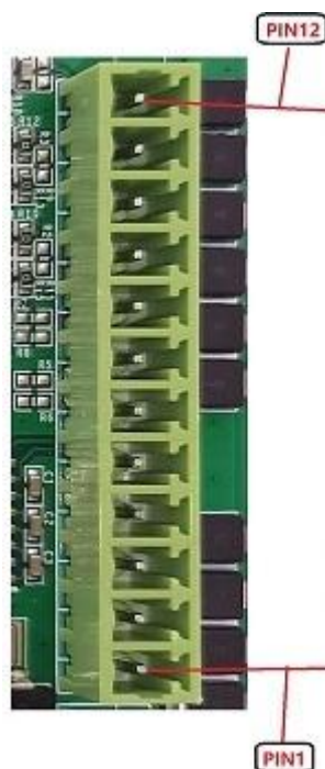
Figure 940: RS232, RS485, CAN
