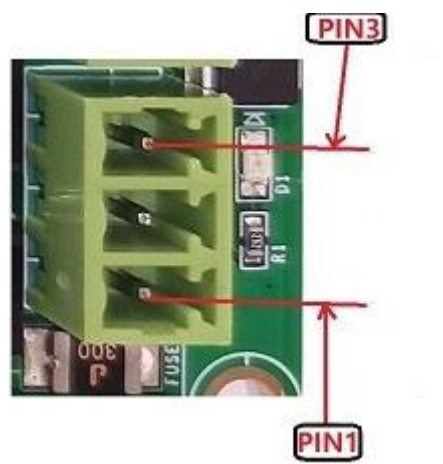
Figure 939: Power Input
