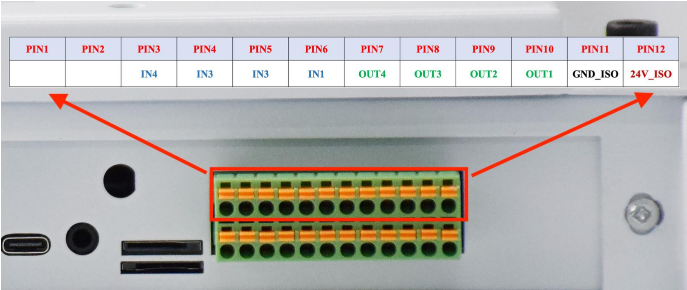
GPIO Connector
