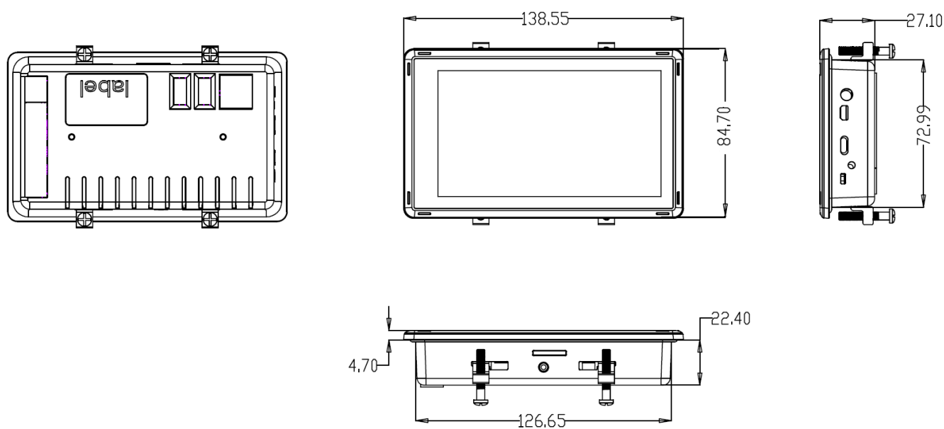
Figure 946: CS12720RA4050P Technical Drawing
